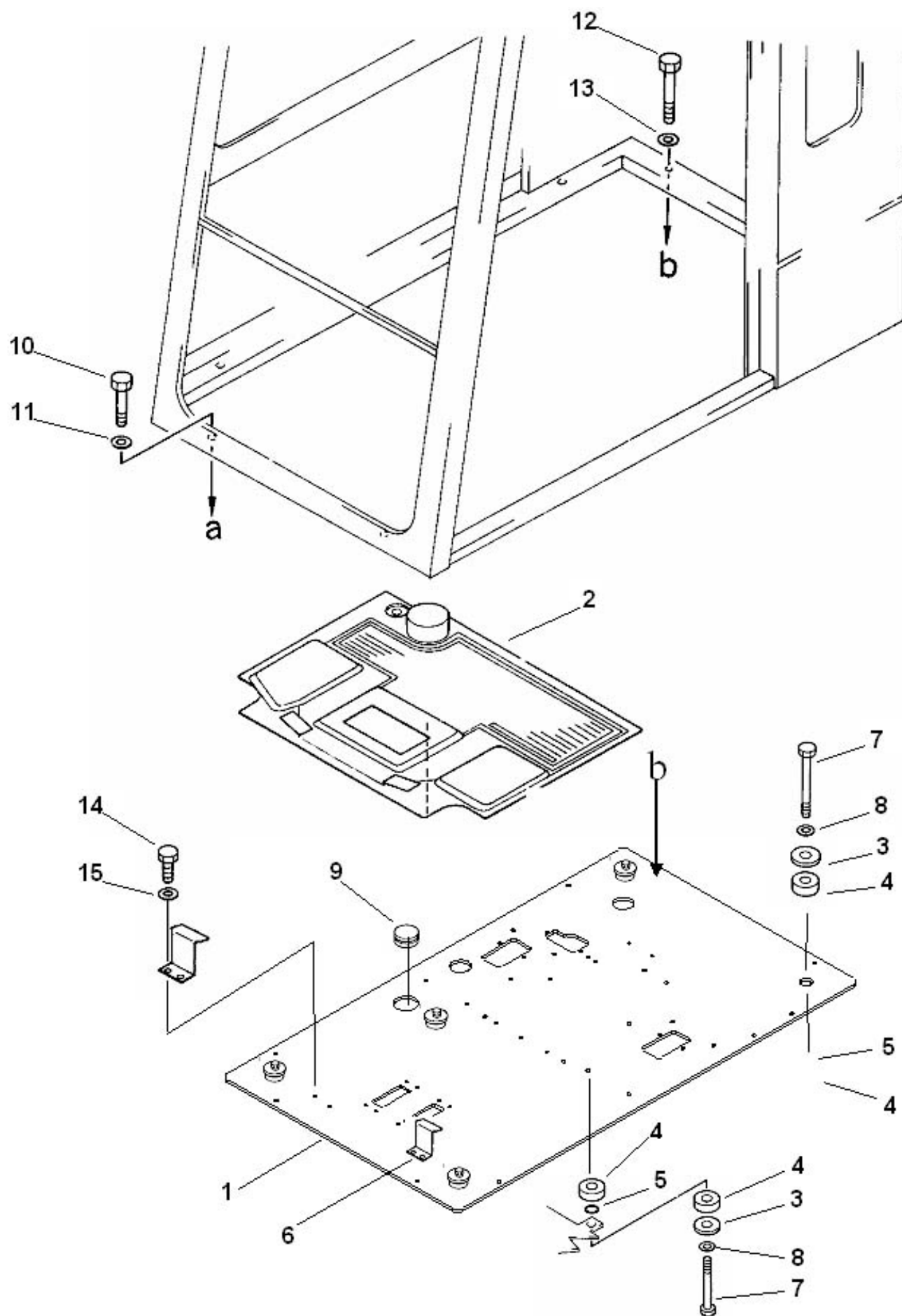
FIG: 5140 OPERATOR'S CAB, FLOOR FRAME
