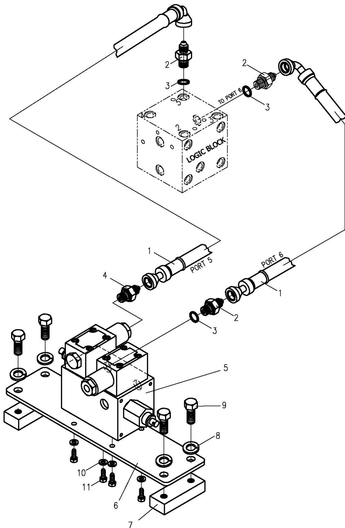
FIG: 4150 PILOT PIPING (5/9) (SWING & BOOM LOGIC)
