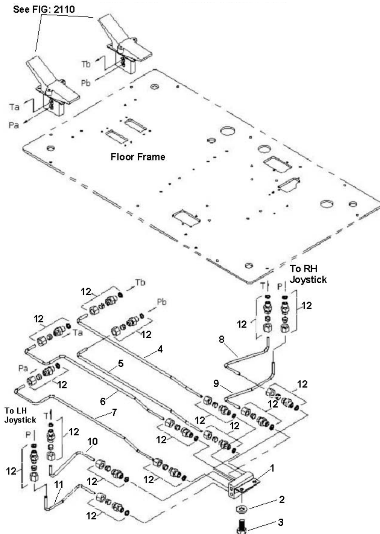
FIG: 4120 PILOT PIPING (2/9)
