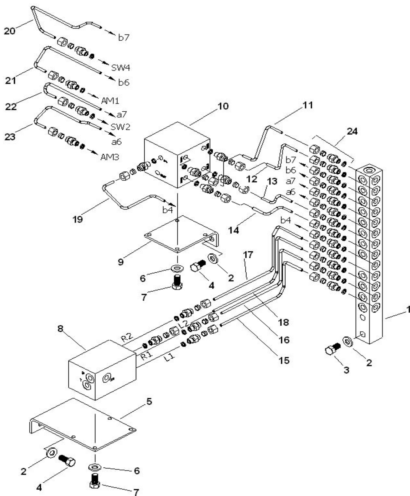
FIG: 4140 PILOT PIPING (4/9)
