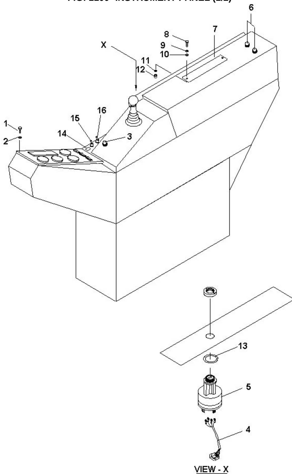
FIG: 1100 INSTRUMENT PANEL (1/2)
