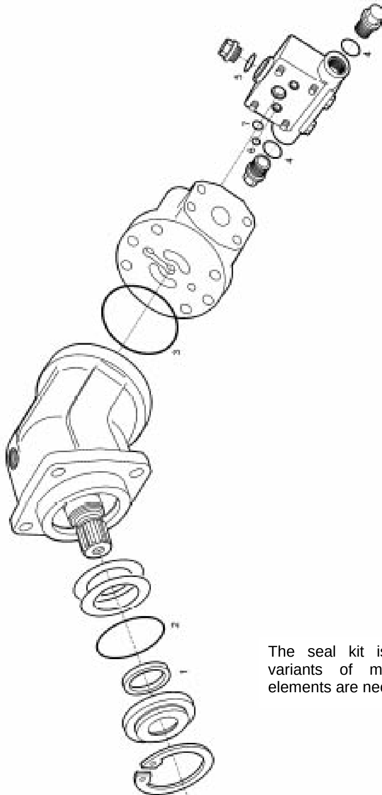
FIG. 11 TRAVEL MOTOR (11/12)
