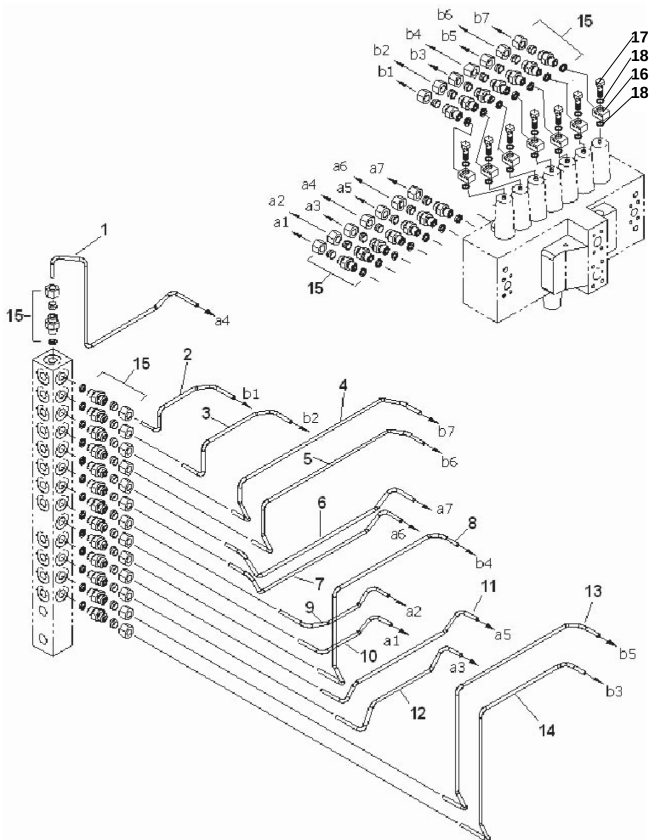
FIG: 4171 PILOT PIPING (7/9) (APPLICABLE FOR SLNO. B16107 AND UP) (AUTO PILOT AIR BLEEDING SYSTEM)
