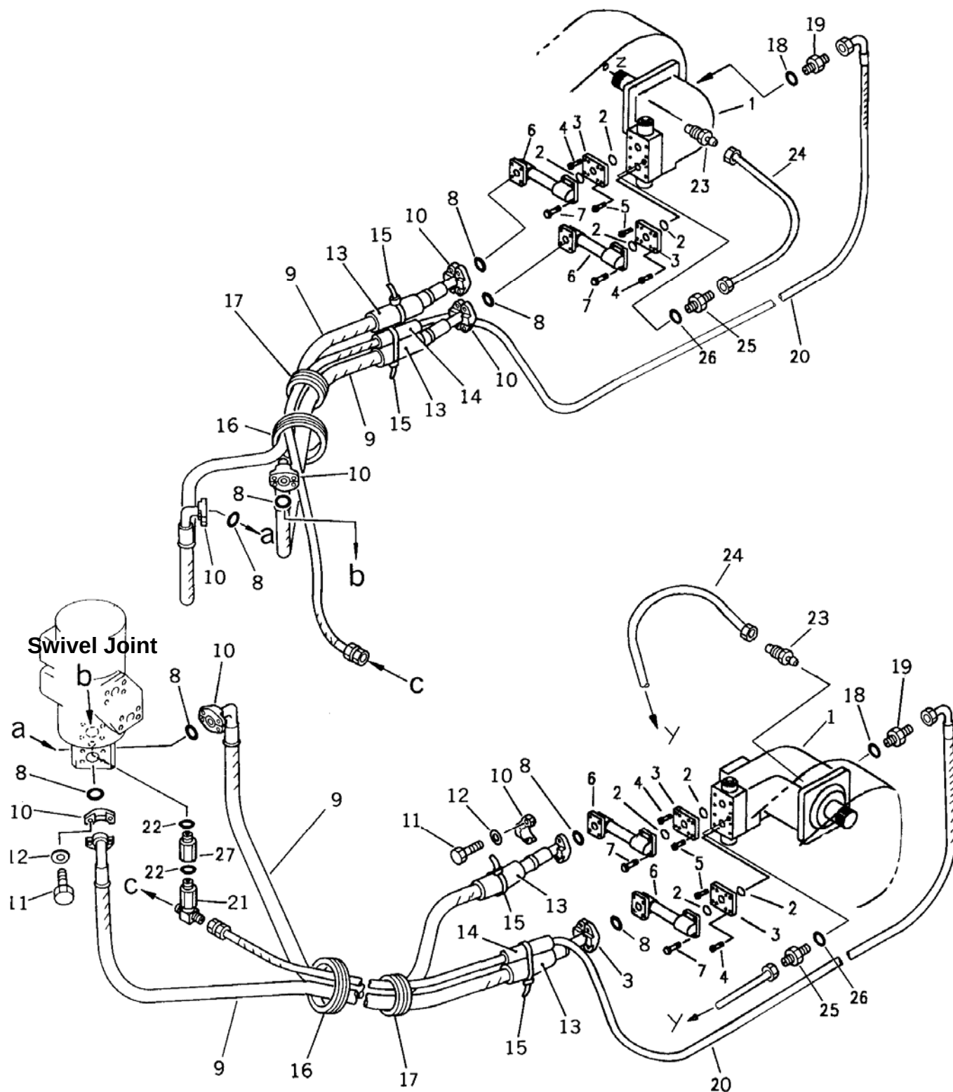
FIG: 2100 HYDRAULIC PIPING (SWIVEL JOINT TO/FROM TRAVEL MO)
