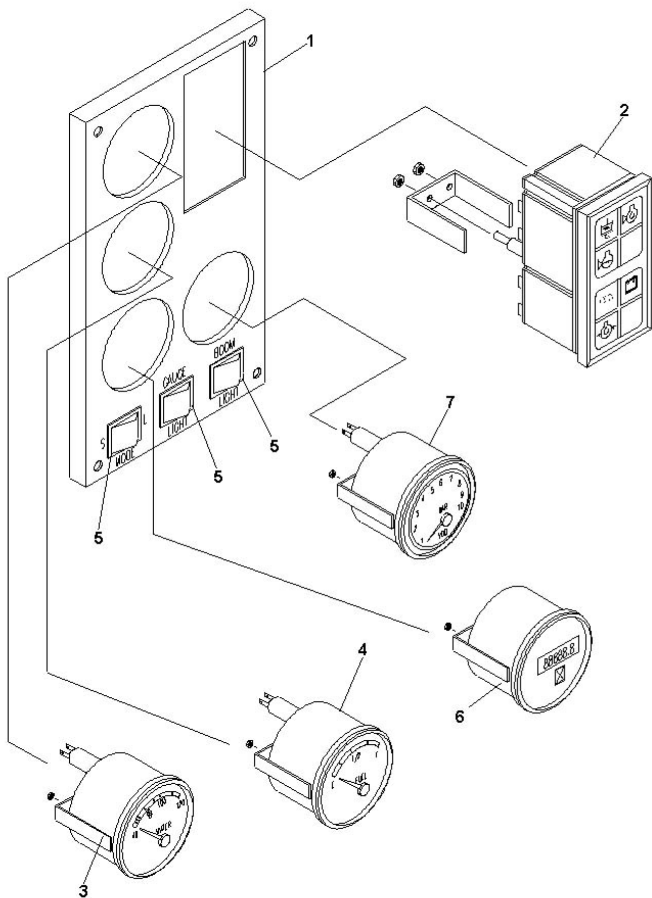
FIG: 1090 MONITOR PANEL AND RELATED PARTS
