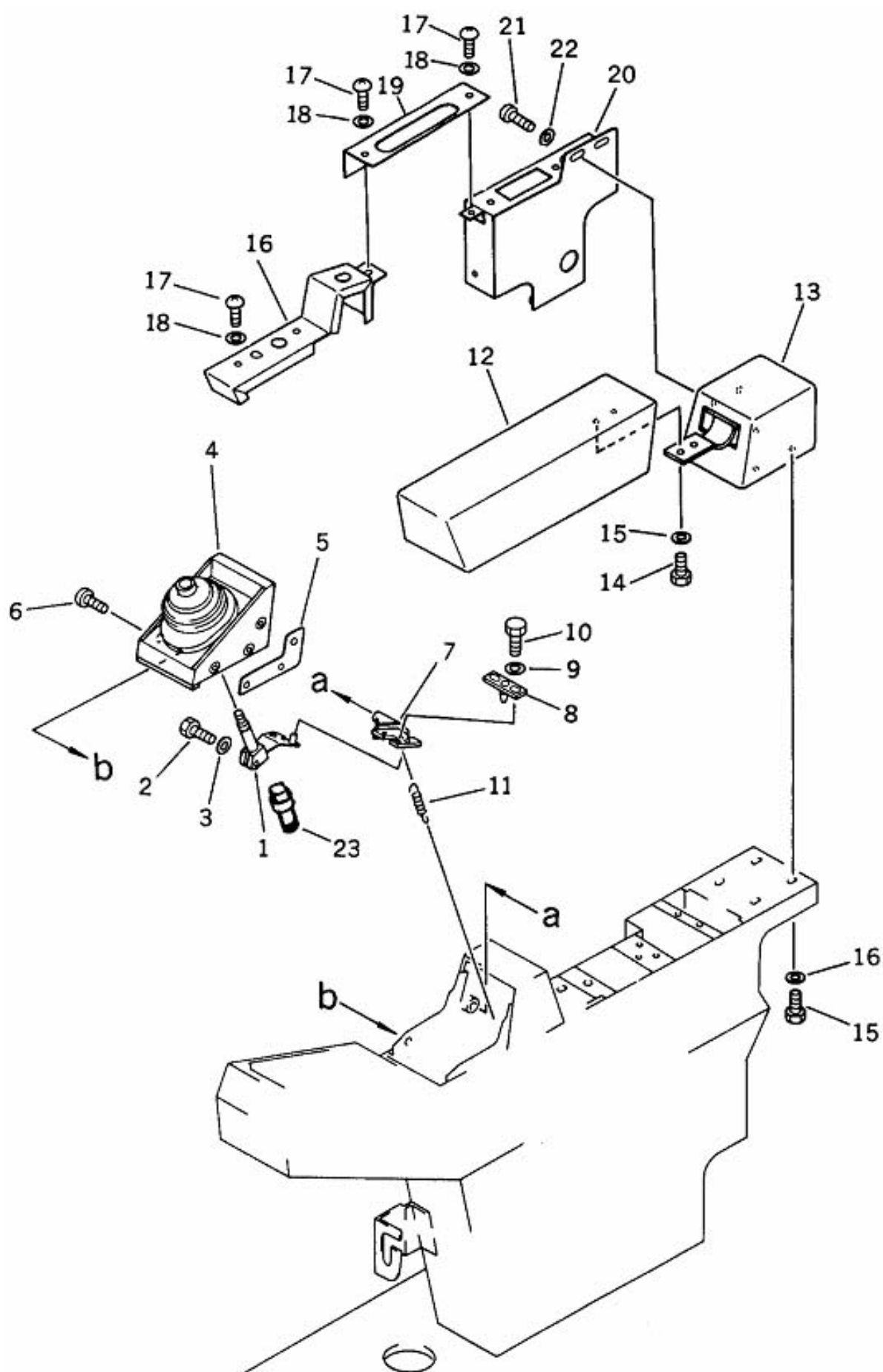
FIG: 4100 WRIST CONTROL AND STAND RH (2/2)
