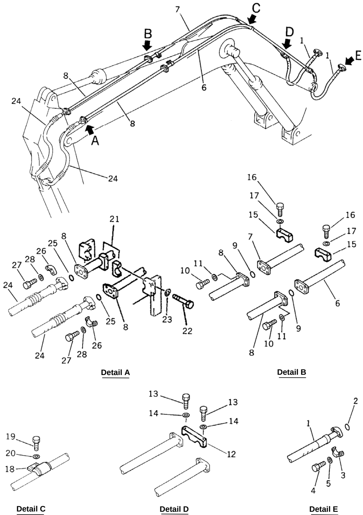
FIG: 6230 HYDRAULIC PIPING (BUCKET CYLINDER LINE)
