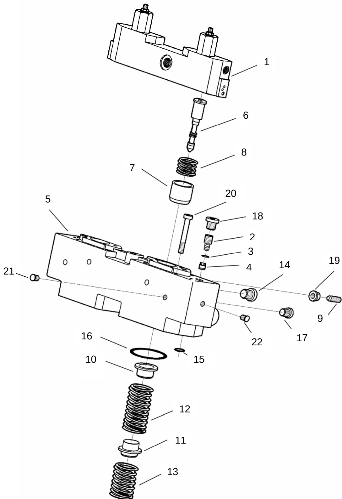
FIG. 26 HYDRAULIC PUMP (7/10)
