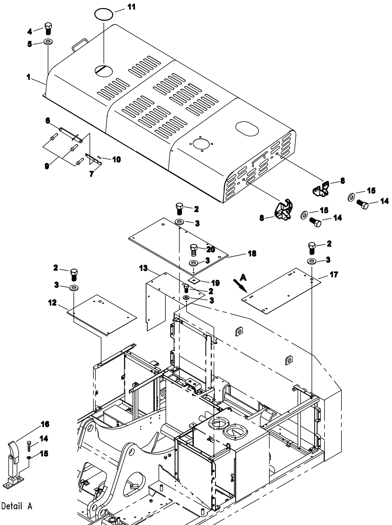
FIG 5040 MACHINERY COMPARTMENT (4/6)
