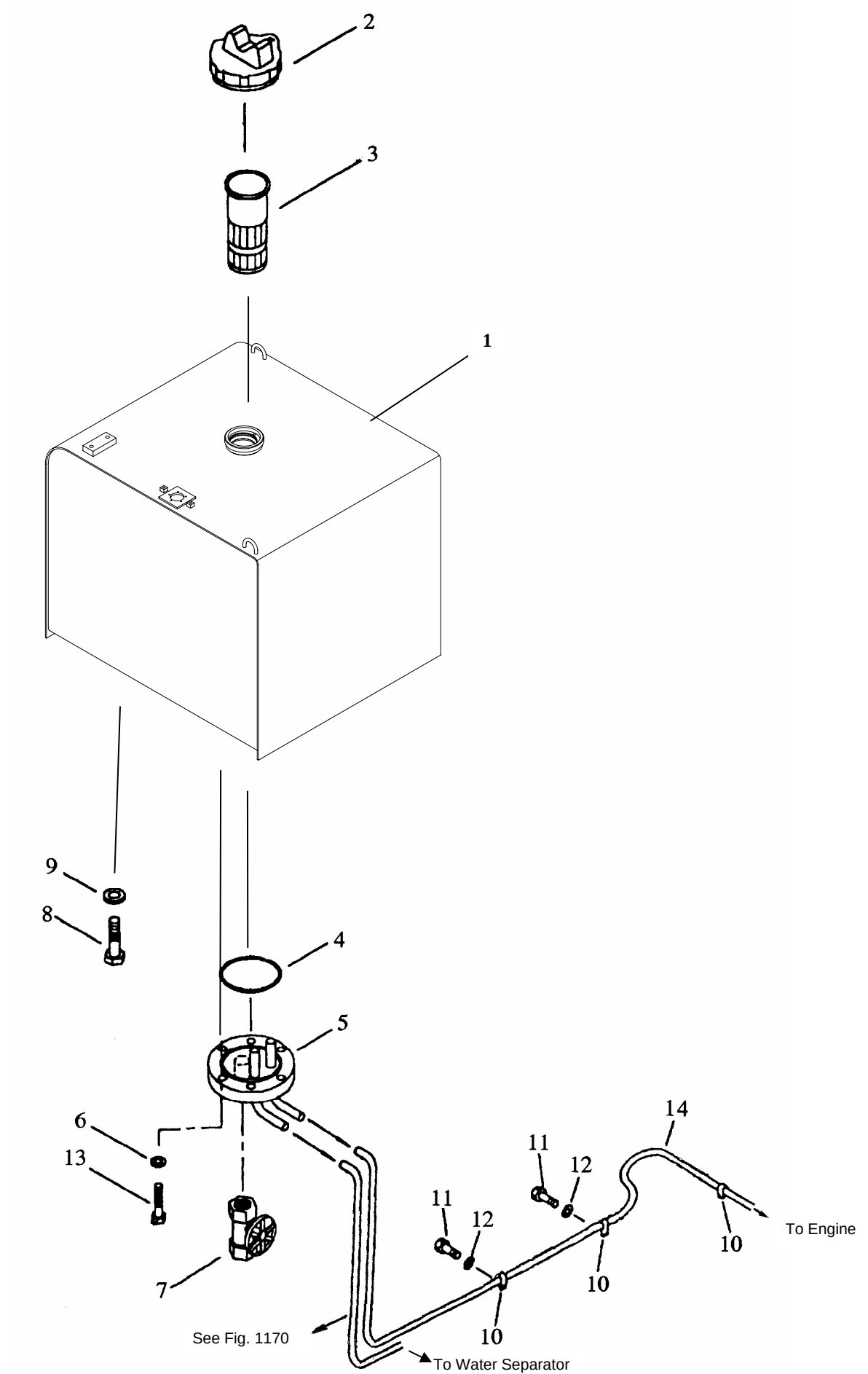
FIG. 1080 FUEL TANK
