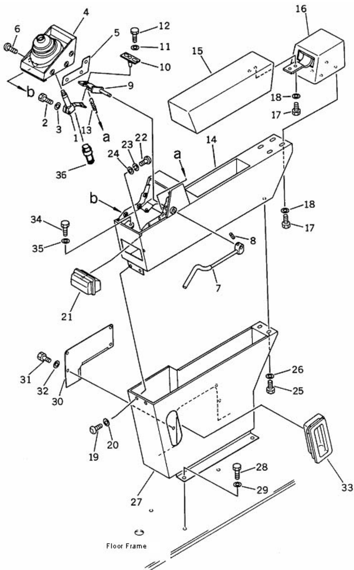
FIG: 4080 WRIST CONTROL AND STAND LH
