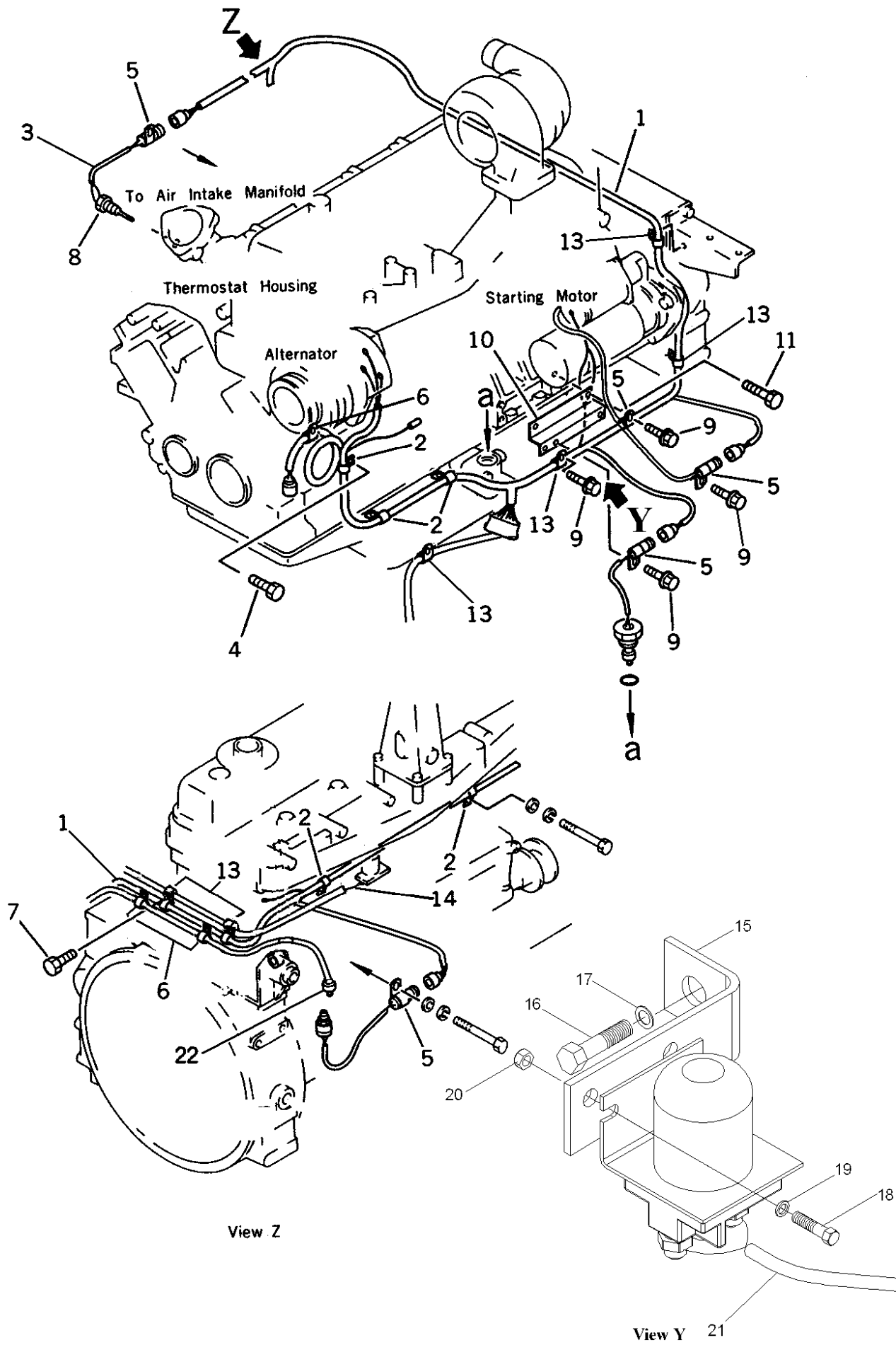
FIG: 1140 ELECTRICAL SYSTEM (WIRING) (2/2)
