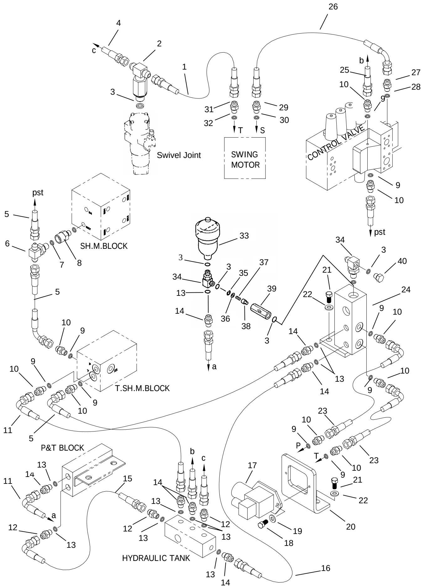
FIG. 4180 PILOT PIPING (8/9)
