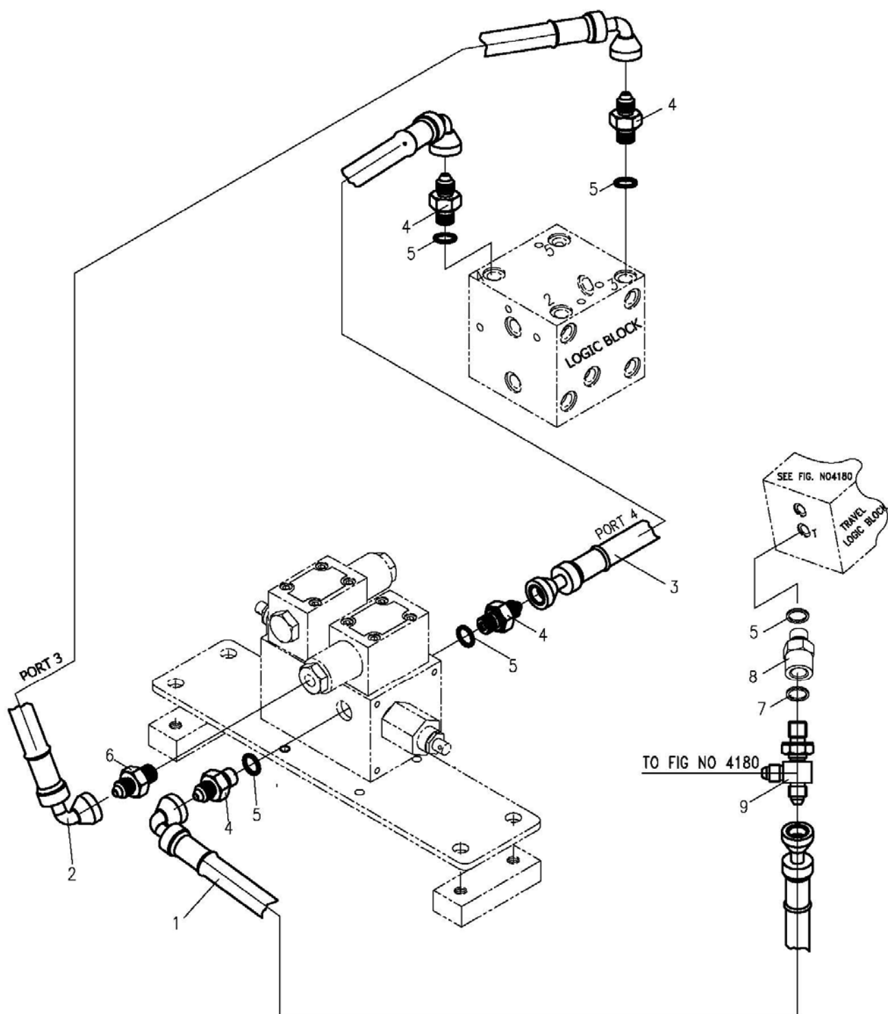
FIG: 4160 PILOT PIPING (6/9) (BUCKET & ARM LOGIC)
