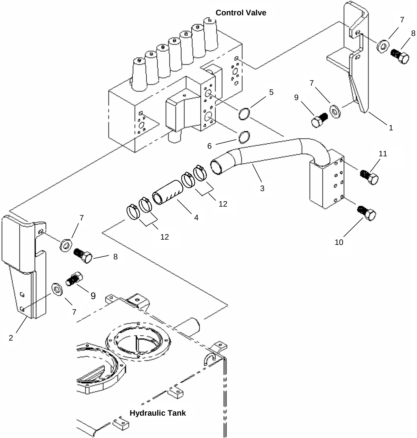
FIG: 6190 HYDRAULIC PIPING (CONTROL VALVE TO TANK (RETURN LINE))
