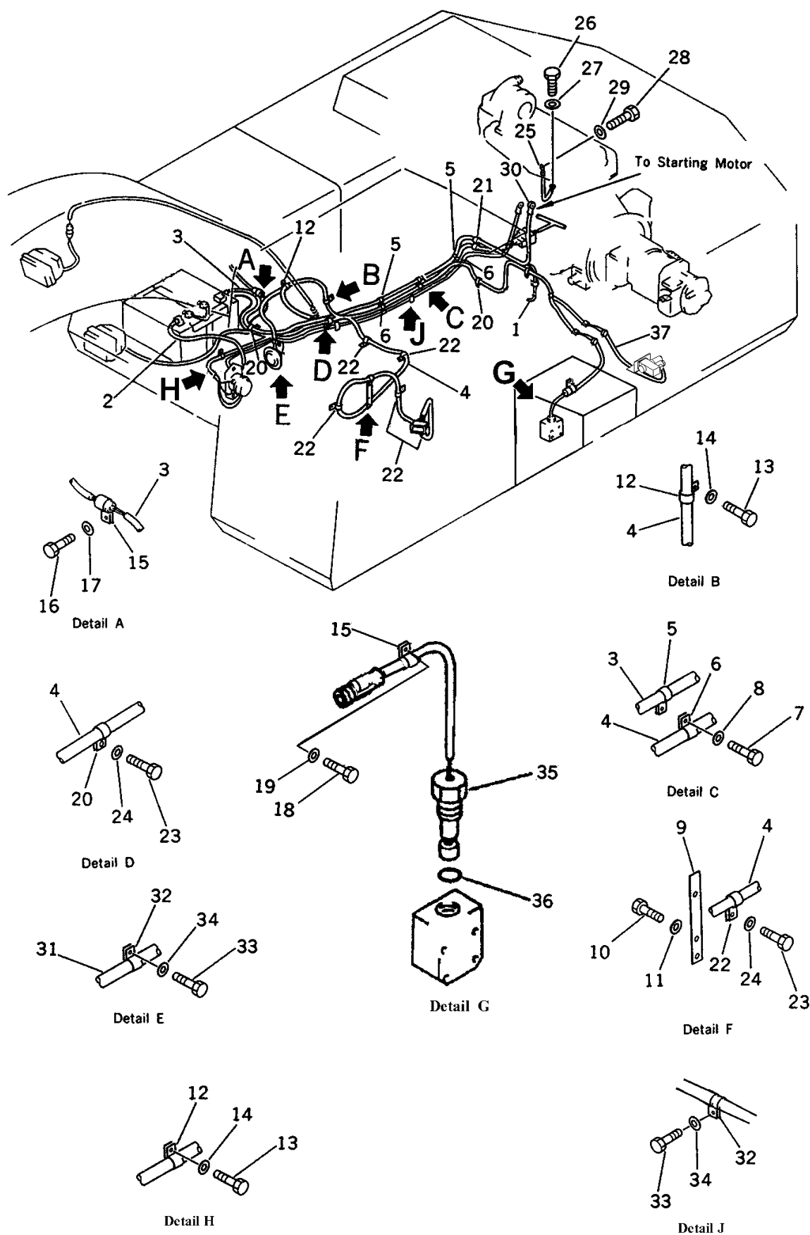
FIG: 1130 ELECTRICAL SYSTEM (WIRING) (1/2)
